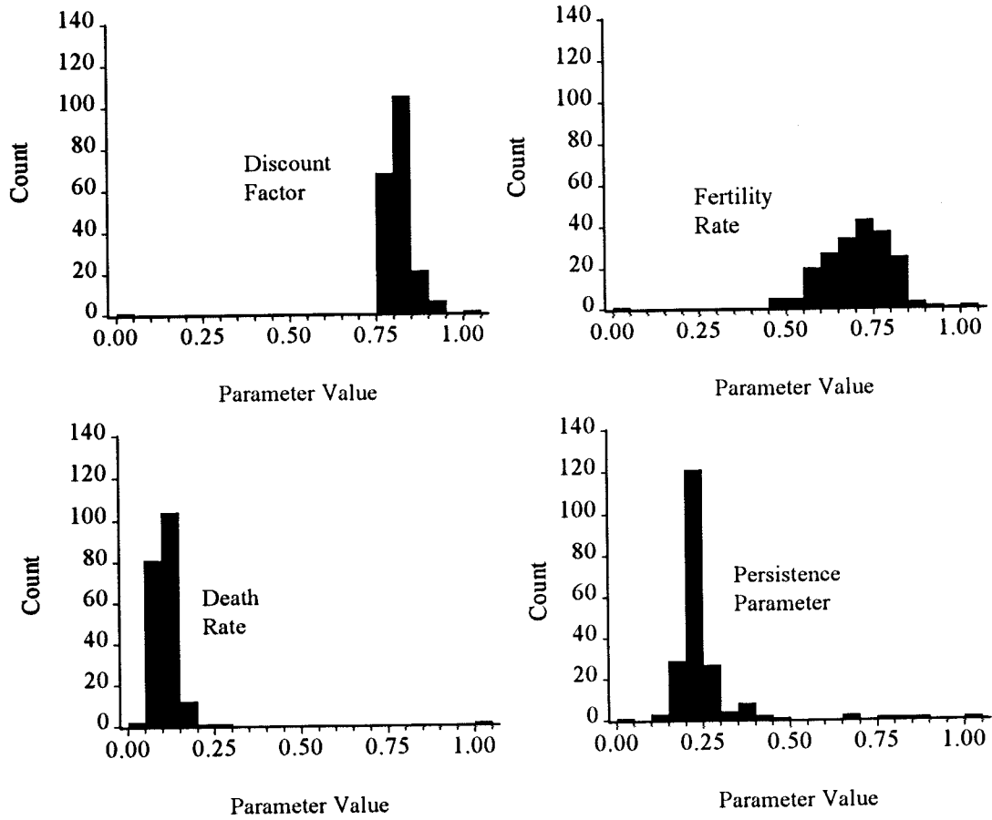
Figure 7 Bootstrap Estimates of Sampling Distributions
