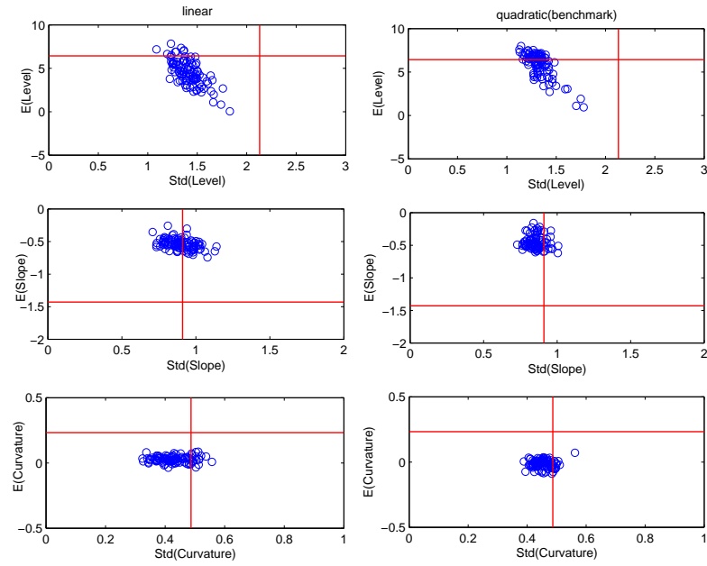
Figure 4: POSTERIOR PREDICTIVE CHECKS II
