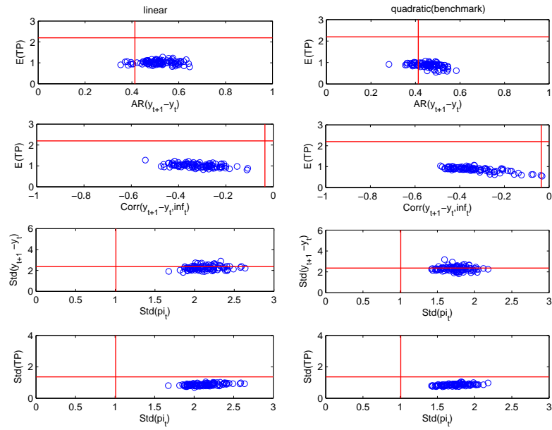
Figure 3: POSTERIOR PREDICTIVE CHECKS I
