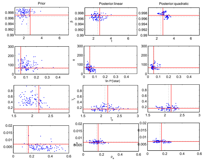
Figure 5: PRIOR-POSTERIOR DRAWS I
