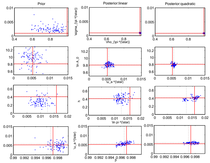
Figure 7: PRIOR-POSTERIOR DRAWS III
