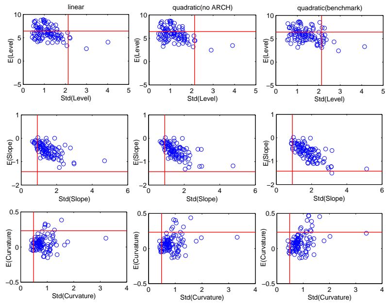
Figure 2: PRIOR PREDICTIVE CHECKS II
