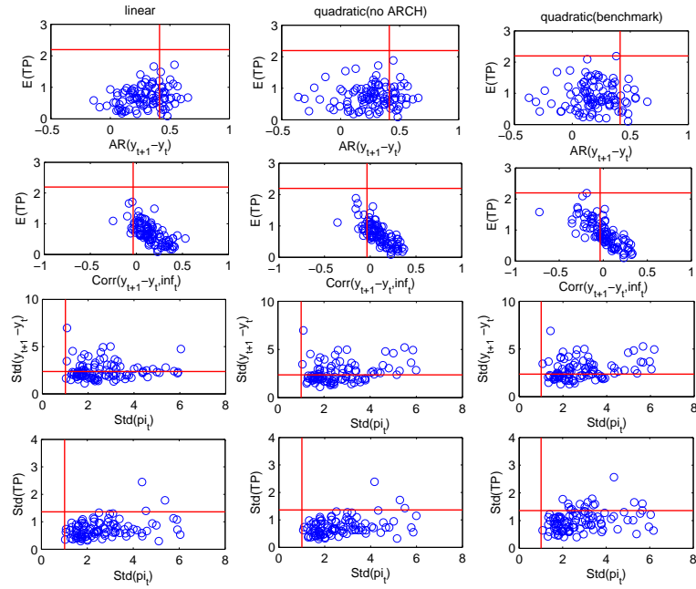
Figure 1: PRIOR PREDICTIVE CHECKS I
