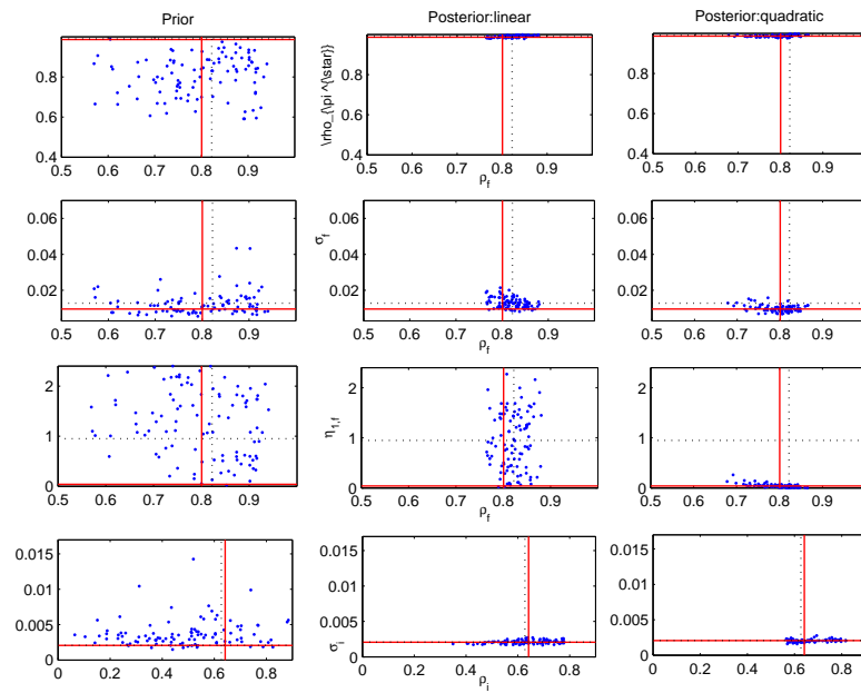
Figure 6: PRIOR-POSTERIOR DRAWS II
