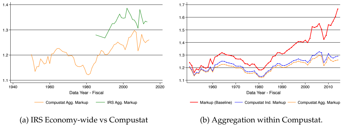
Figure B.5: Panel (a): Markups based on aggregates: IRS (Total Business Receipts/Total Cost of Goods sold and Compustat (Total Sales/ Total Cost of Goods Sold) and \theta = 0.85 . Panel (b): repeat Compustat aggregate, and compare to base-line measure, M_t firm-level sales-share weighted markup, and Compustat aggregate (Compustat Ind. Markup) based on aggregate industry-wide markups, using industry sales weights.
