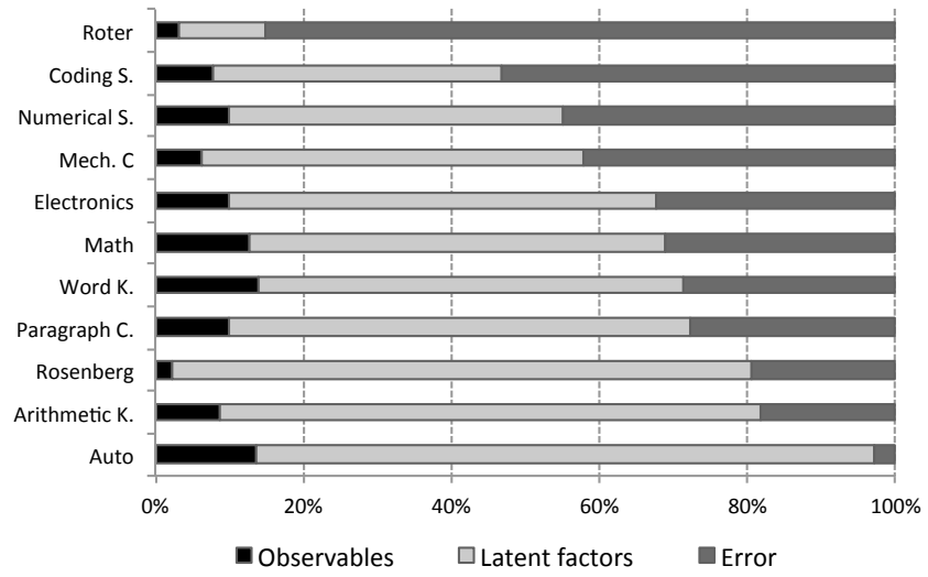
Figure 4: Variance Decomposition
