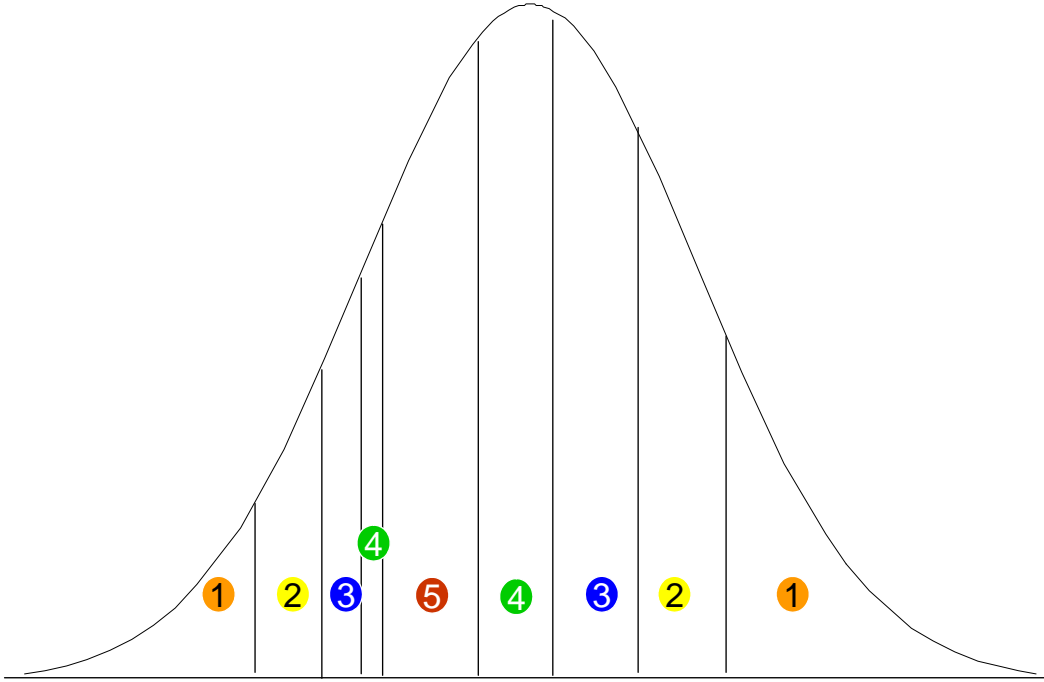
Figure 6: An example of the optimal strategy
