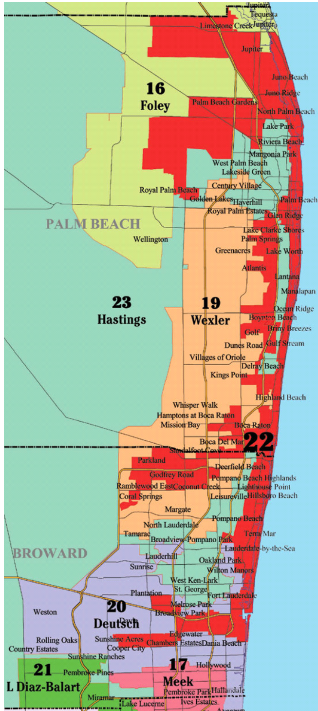
Figure 1: Florida 16th to 23rd Congressional Districts
