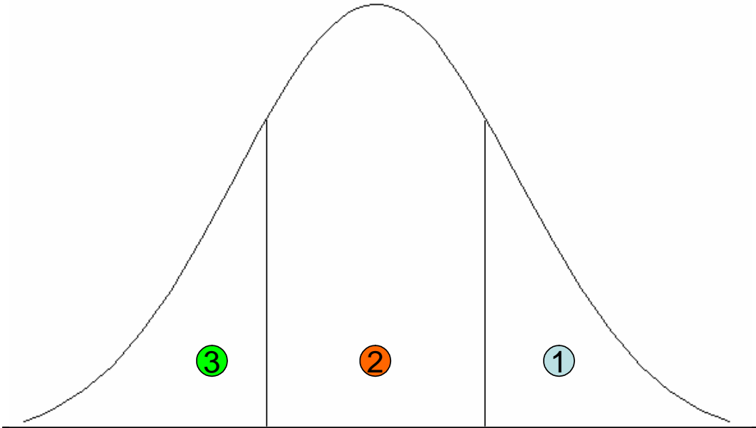
Figure 5: Proposition 2 rules out this strategy
