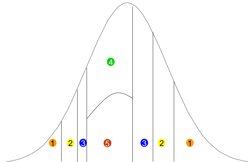
Figure 3: Slices and Parfaits
