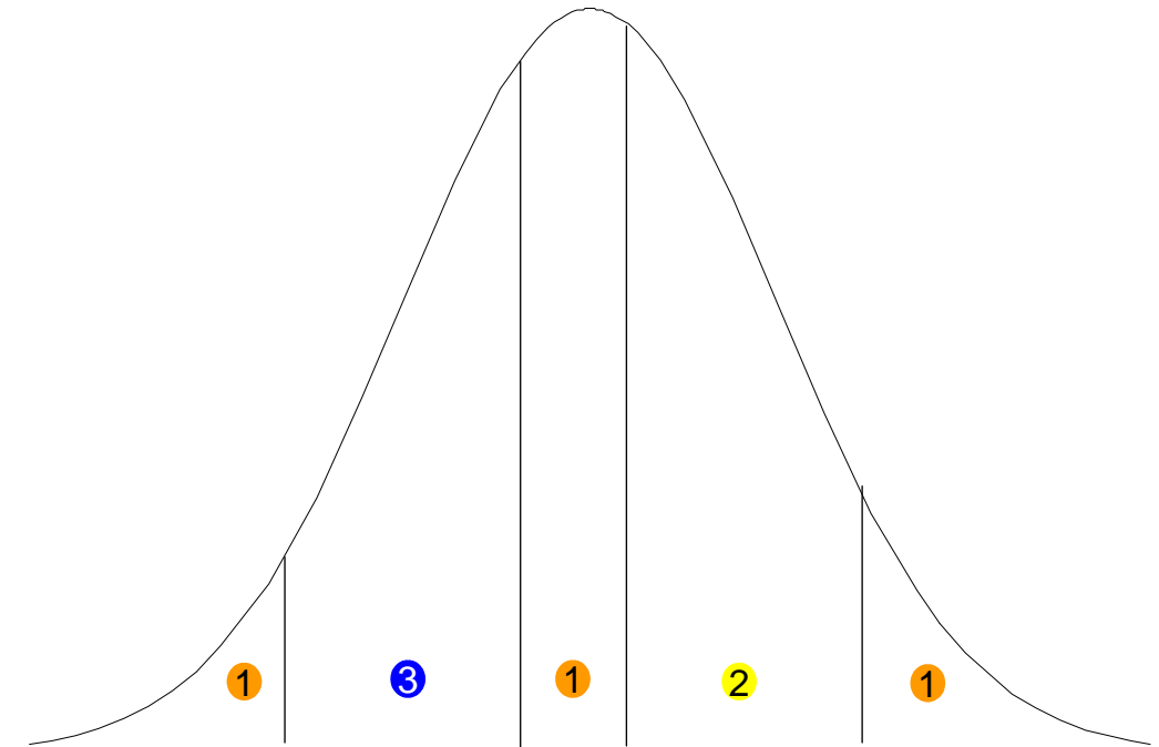
Figure 4: An example of a strategy ruled out by Lemma 3.
