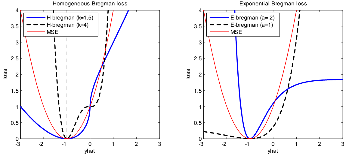
Figure 1: Examples of Bregman loss functions for \hat{y} \in [-3, 3] when y = -1 . The left panel presents examples of “homogeneous Bregman” loss functions of the form L(y, \hat{y}) = |y|^a - |\hat{y}|^a - \text{sgn}(\hat{y}) a |\hat{y}|^{a-1} (y - \hat{y}) , for a > 1 . The right panel presents examples of “exponential Bregman” loss functions of the form L(y, \hat{y}) = 2a^{-2} (\exp\{ay\} - \exp\{a\hat{y}\}) - 2a^{-1} \exp\{a\hat{y}\} (y - \hat{y}) , for a \neq 0 . Both of these families nest MSE ( k = 2 in the former case and a \rightarrow 0 in the latter).
