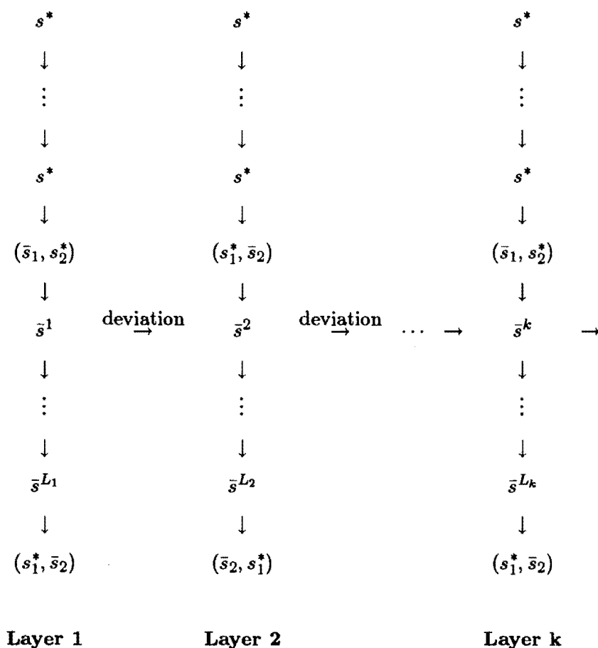
Figure 3: Equilibrium paths in an alternating move game.
