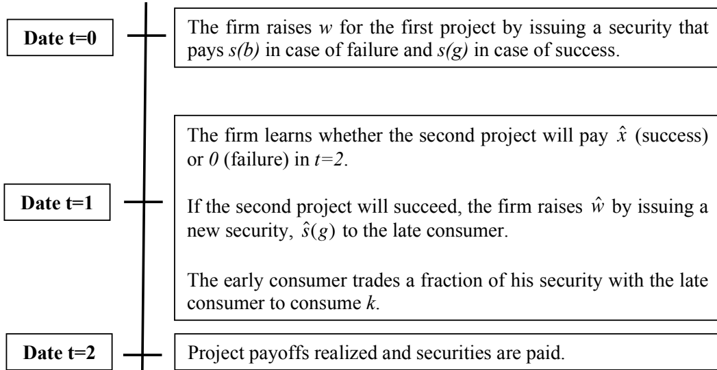
Figure 1: Timing Model with Capital Markets
