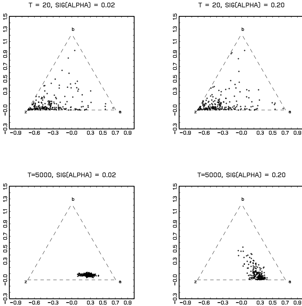
Figure 1: Spectral decomposition of output at frequency 1/12 cycles per quarter based on artificial observations generated from DSGE model. Sample size: T = 20 and T = 5000 . Prior standard errors of \alpha are 0.02 and 0.20, respectively. Dots correspond to 200 draws from VAR posterior distribution. V indicates posterior mean of VAR.
